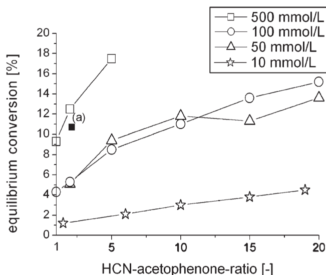
Figure 2. Acetophenone cyanohydrin synthesis in one-phase-system consisting of a mixture of ethanol and citrate buffer pH 4.0: (-☆-) 10 mmol/L acetophenone: 100 % (v/v) buffer, (-△-) 50 mmol/L acetophenone: 25 % (v/v) ethanol, 75 % (v/v) buffer, (-○-) 100 mmol/L acetophenone: 35 % (v/v) ethanol, 65 % (v/v) buffer, (-□-) 500 mmol/L acetophenone 50 % (v/v) ethanol, 50 % (v/v) buffer. Reaction conditions: 5 °C, 50–500 mmol/L citrate buffer pH 4.0/ethanol, 400 rpm. Equilibrium constant: K = 0.0006 \text{ L/mmole} . Due to the determination of the thermodynamic equilibrium no enzyme was required (reaction yielding the racemate). [a] [Bühler et al. 2003] [12] – 200 mmol/L acetophenone, 400 mmol/L hydrogen cyanide (ratio 1:2) in diisopropyl ether with immobilized MeHNL on nitrocellulose (pure organic one-phase system).
