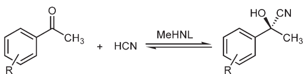
Figure 1. (S)-Acetophenone cyanohydrin synthesis using the hydroxynitrile lyase from Manihot esculenta (MeHNL).
